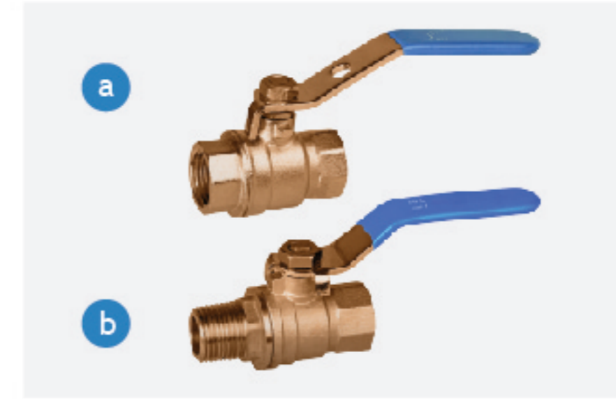
BALL VALVE - Kelas: PN10/PN16 - Sistem sambungan: ulir standar BSPT/ISO 7/1 - Ukuran: a. Female x Female: 1/4" - 4" b. Male x Female: 1/2" - 1" - Class: PN10/PN16 - Connection system: thread standard BSPT/ISO 7/1 - Size: a. Female x Female: 1/4" - 4" b. Male x Female: 1/2" - 1"
